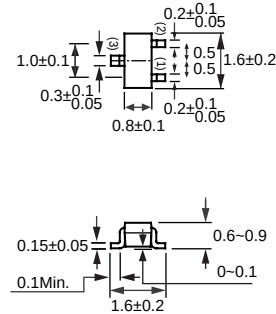
SC-75/SOT-416
