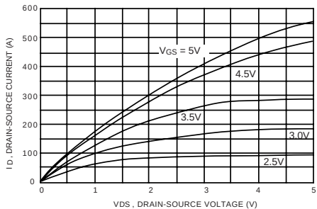
Figure 1. On-Region Characteristics
