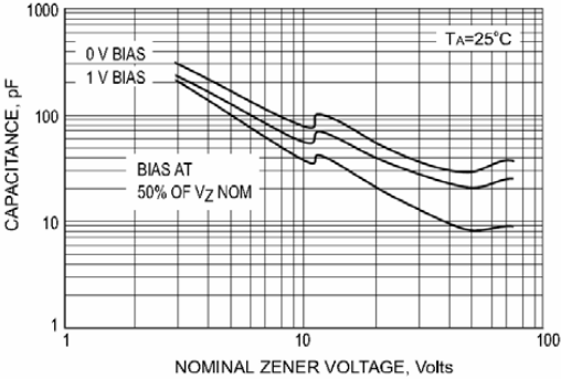
Fig.2 TYPICAL CAPACITANCE
