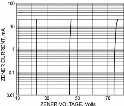
Fig.4 ZENER BREAKDOWN CHARACTERISTICS
