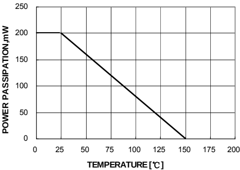
Fig.1 POWER DISSIPATION VS. AMBIENT TEMP.
