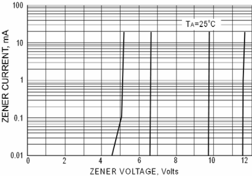
Fig.3 ZENER BREAKDOWN CHARACTERISTICS
