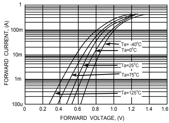
FIG. 1 - FORWARD CHARACTERISTICS
