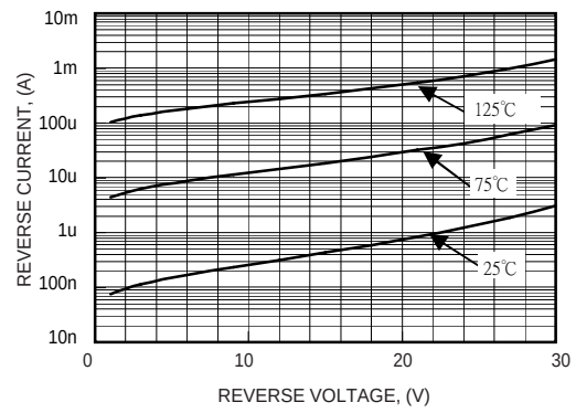
FIG. 2 - REVERSE CHARACTERISTICS
